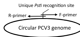
Fig. 1. Sketch of PCV3 genome amplification using tail-to-tail overlapping primers that were designed to have a unique type II restriction endonuclease, Pst I recognition site in the overlapping region that was later used for full-genome cloning. This is to ensure that the genome amplified is from the same genome, and not from separate genomes.
